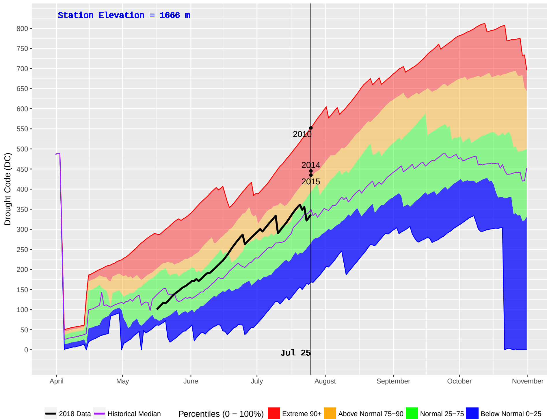
BALDFACE (221) : Historical (1992–2016) and Current (2018) Noon Drought Code (DC)
