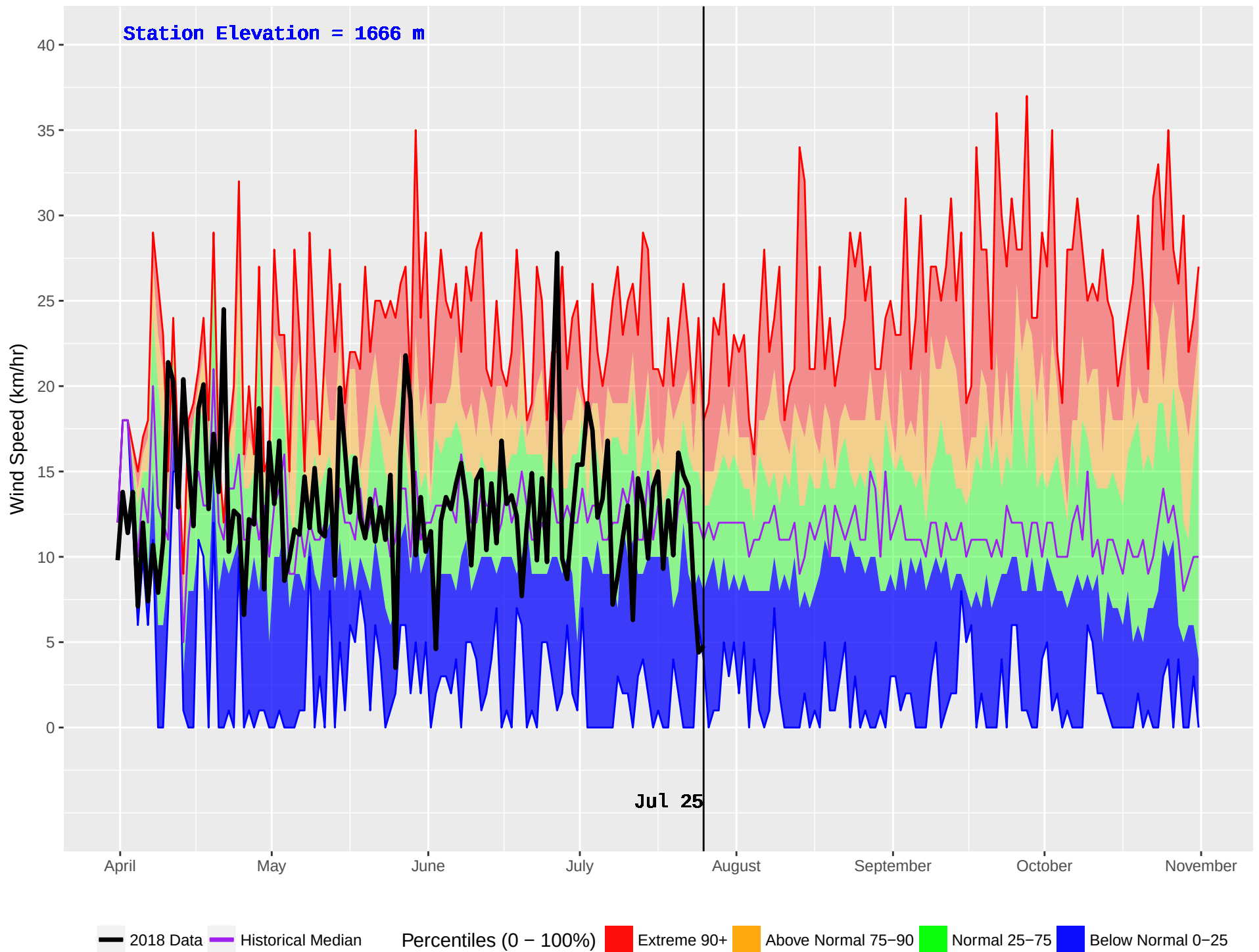
BALDFACE (221) : Historical (1992–2016) and Current (2018) Noon Wind Speed
