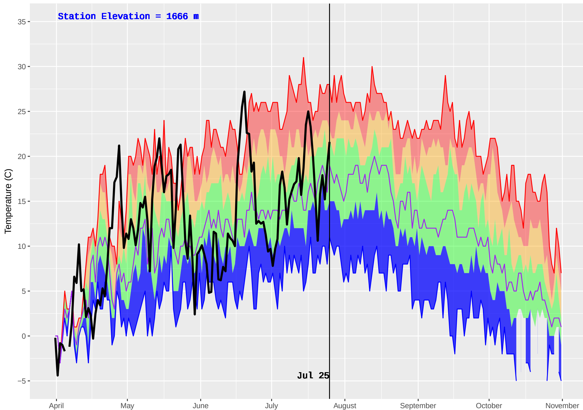
BALDFACE (221) : Historical (1992–2016) and Current (2018) Noon Temperature
