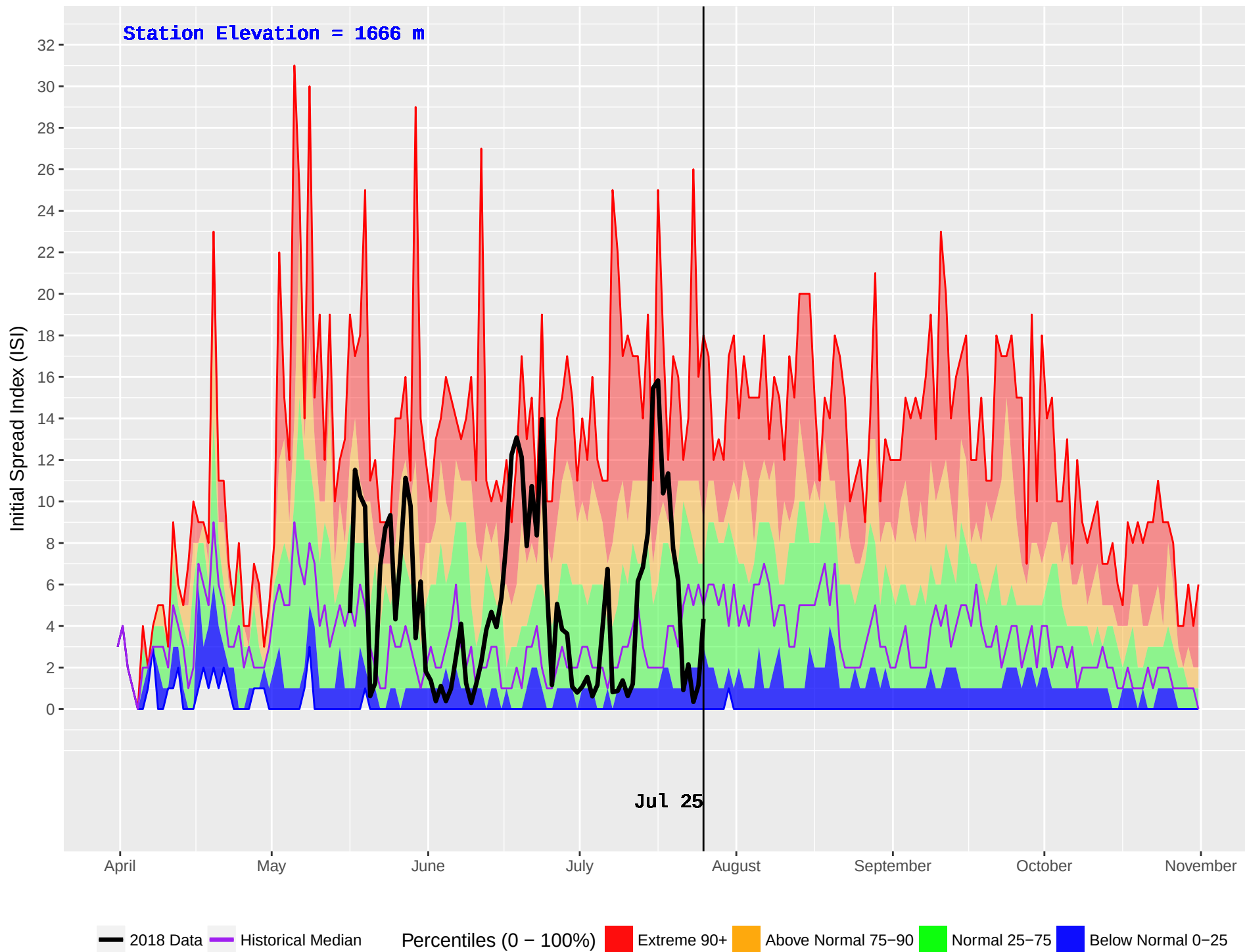
BALDFACE (221) : Historical (1992–2016) and Current (2018) Noon Initial Spread Index (ISI)
