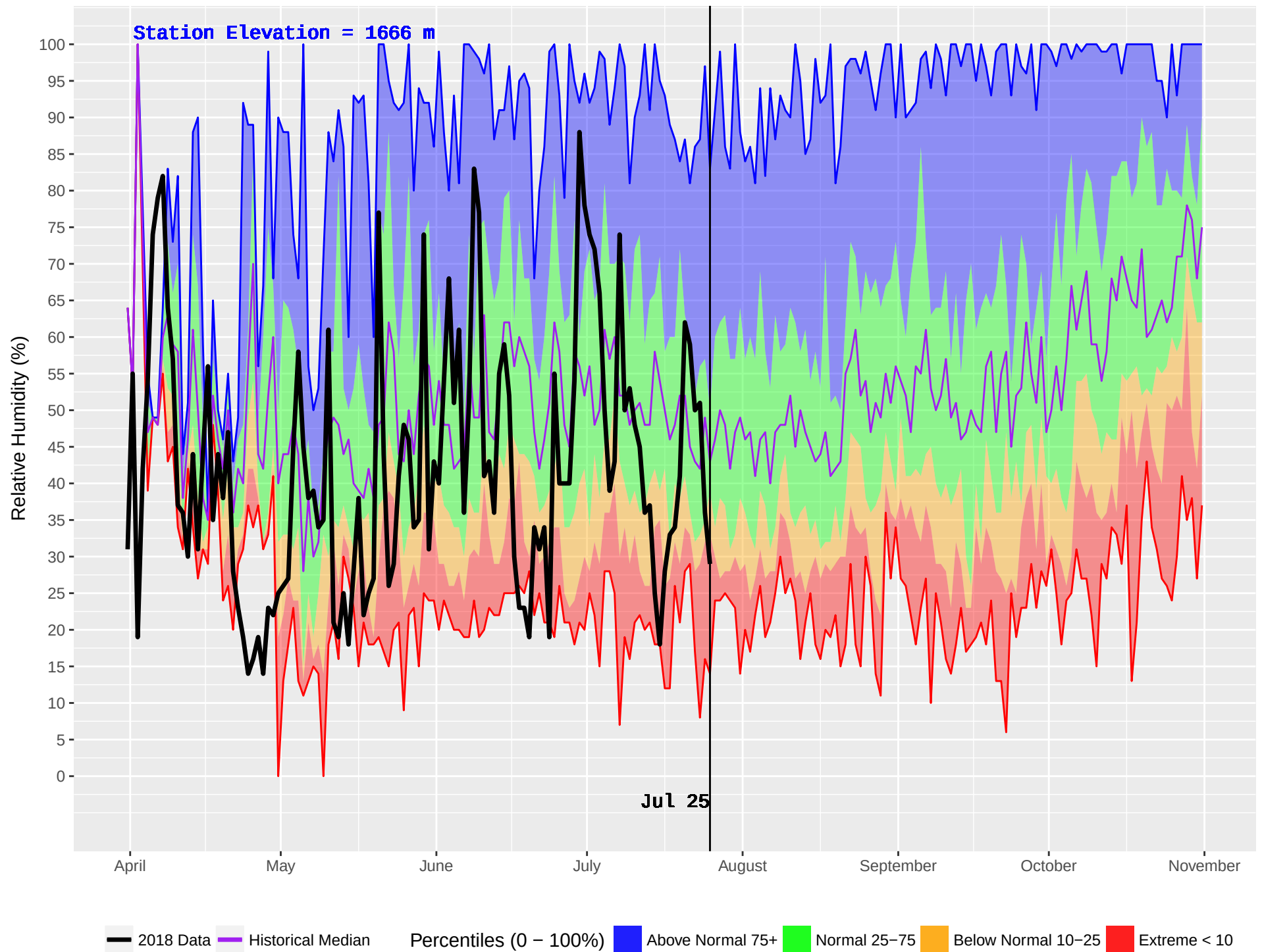
BALDFACE (221) : Historical (1992–2016) and Current (2018) Noon Relative Humidity
