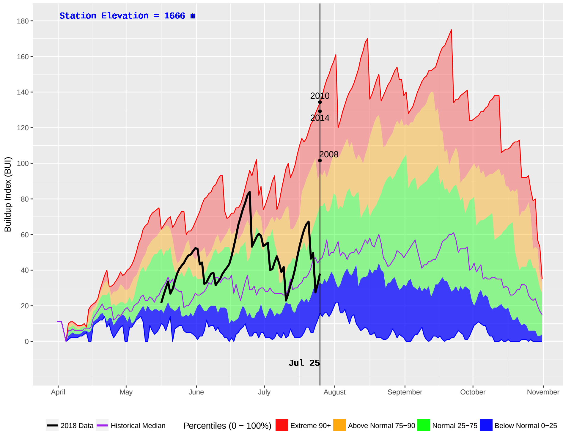
BALDFACE (221) : Historical (1992–2016) and Current (2018) Noon Buildup Index (BUI)
