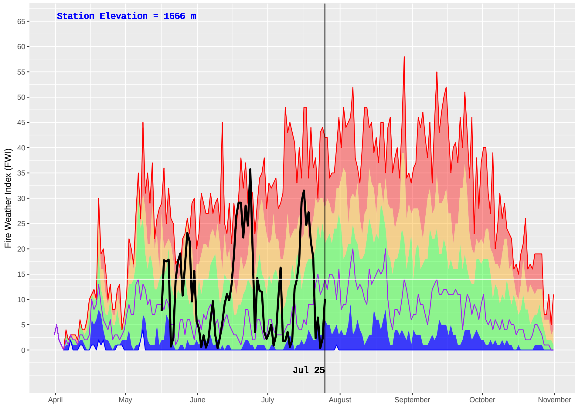
BALDFACE (221) : Historical (1992–2016) and Current (2018) Noon Fire Weather Index (FWI)
